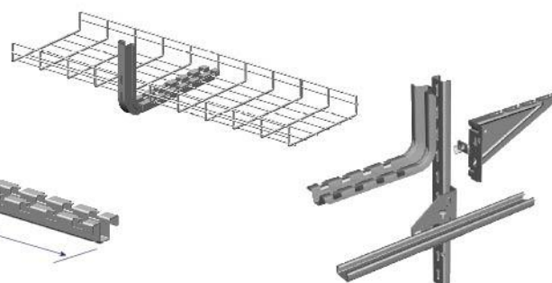
BM-LB L Bracket
